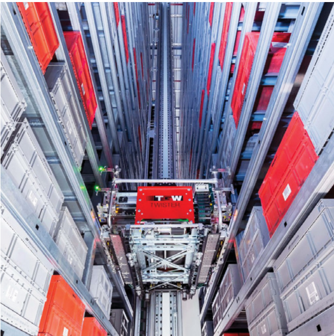
Miniload Systems
